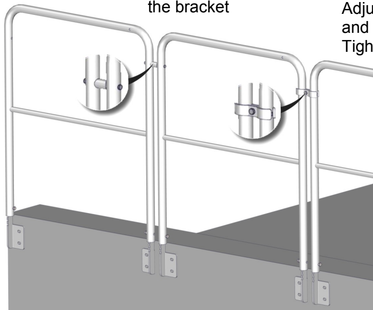
Thread the railing on to the bracket
